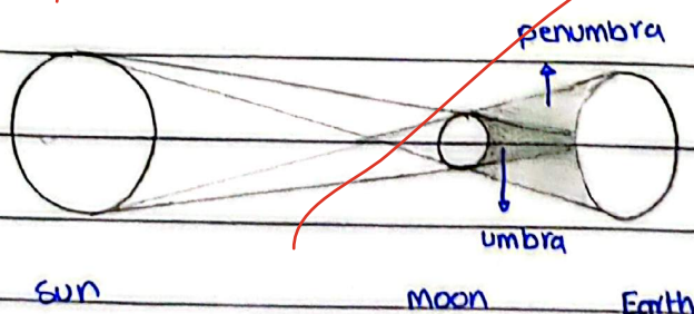
Solar Eclipse
