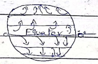
Coriolis force effect.
