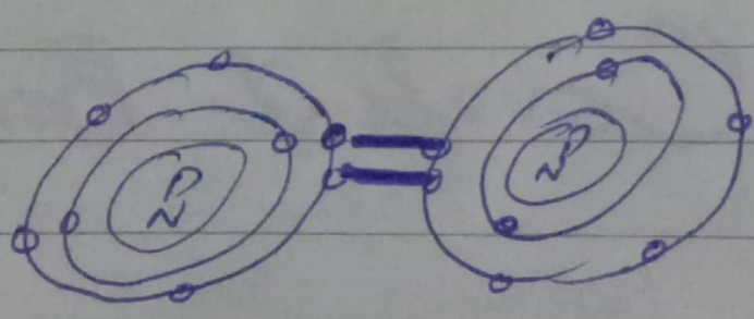
Oxygen Atomic Number = 8
