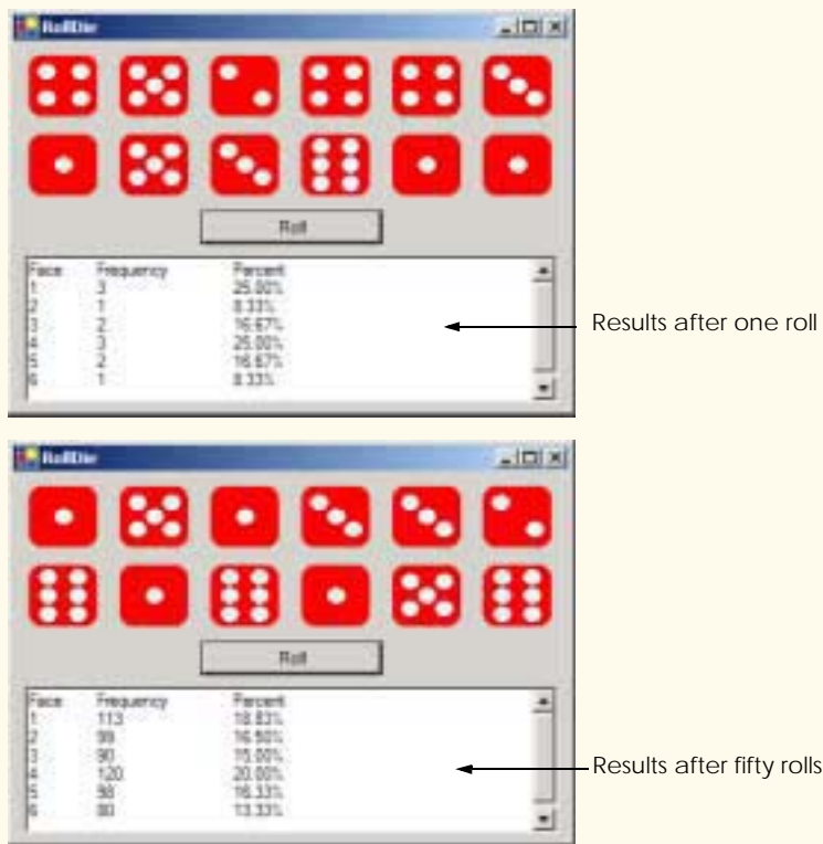
Fig. 7.6 Using arrays to eliminate a switch structure. (Part 3 of 3.)
