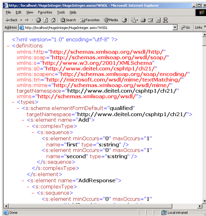
Fig. 21.2 Service description for a Web service.
