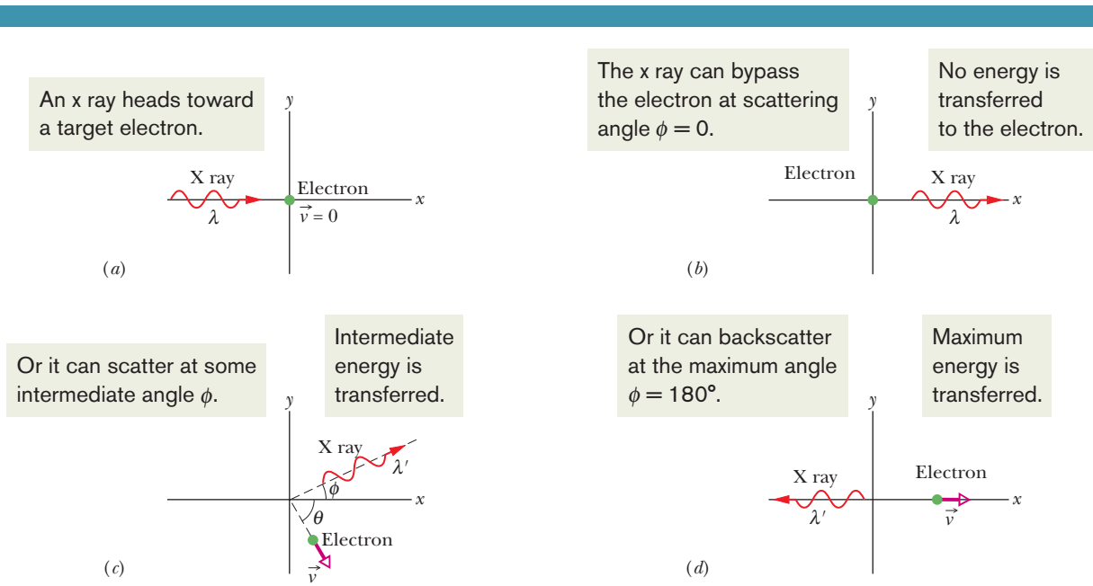
Figure 38-5 (a) An x ray approaches a stationary electron. The x ray can (b) bypass the electron (forward scatter) with no energy or momentum transfer, (c) scatter at some intermediate angle with an intermediate energy and momentum transfer, or (d) backscatter with the maximum energy and momentum transfer.
