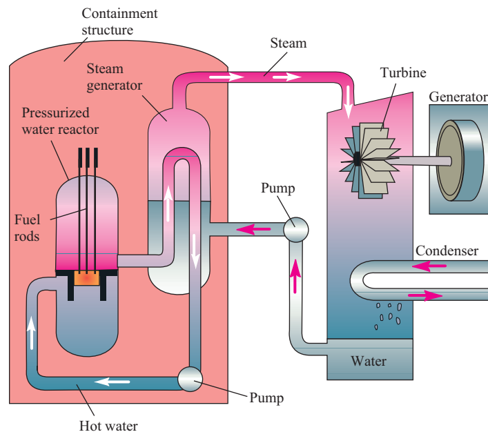
FIGURE 19.23 Pressurized water nuclear reactor. Water is superheated and pressurized as it flows through the reactor core. Heat is transferred to nonpressurized water in the steam generator. The steam drives the turbogenerator to produce electricity.
