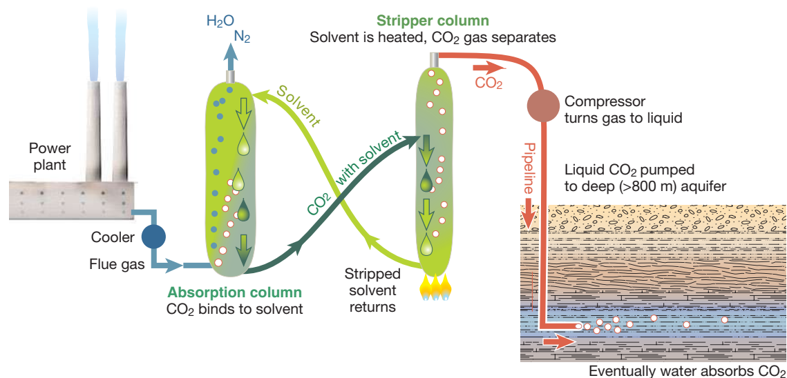
FIGURE 15.26 One method of carbon capture and storage uses a liquid solvent, such as ammonia, to capture CO 2 . Steam and nitrogen are released, and the CO 2 is compressed and pumped to deep aquifers for permanent storage.
