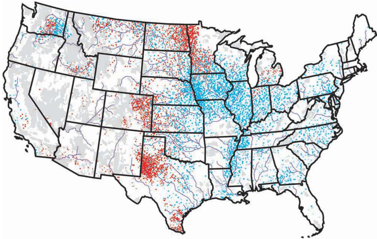
FIGURE 10.8 More than 43.7 million ha (108 million acres) in the United States are subjected to excess wind (red) or water (blue) erosion each year.
