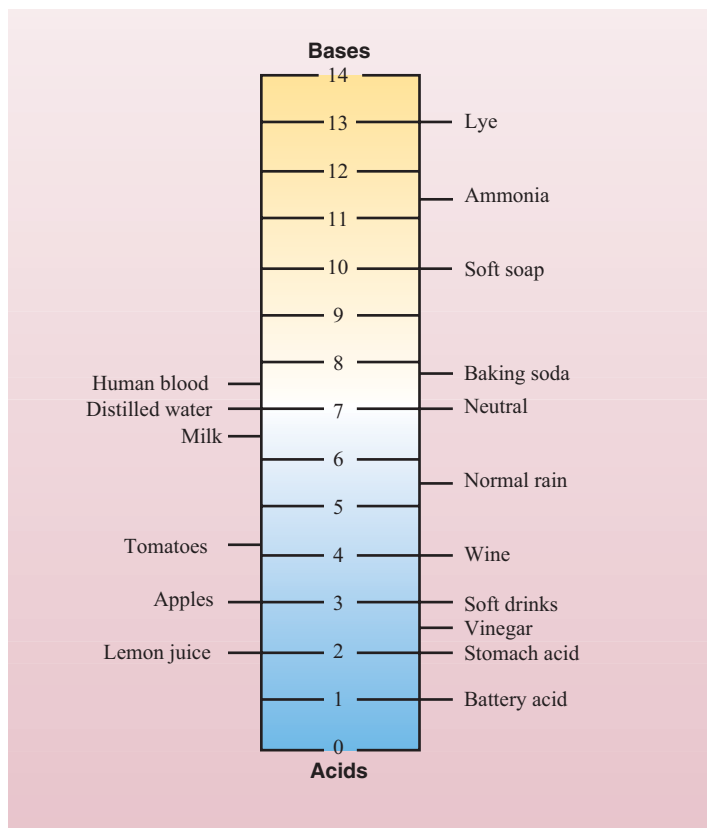
FIGURE 3.4 The pH scale. The numbers represent the negative logarithm of the hydrogen ion concentration in water.
