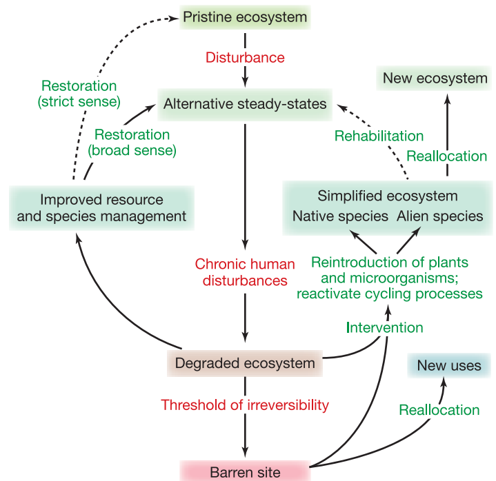
A model of ecosystem degradation and potential management options. Source: Data from Walker and Moral, 2003.
