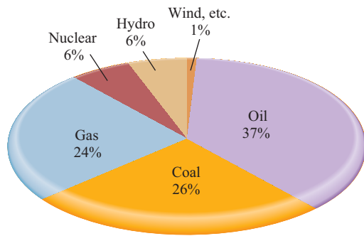
FIGURE 19.3 Worldwide commercial energy consumption. This does not include energy collected for personal use or traded in informal markets. Source: Data from British Petroleum, 2006.
