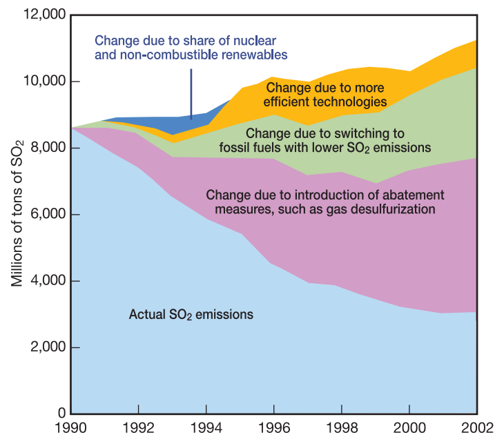
Sulfur dioxide emission reductions in Europe, 1990–2002.
