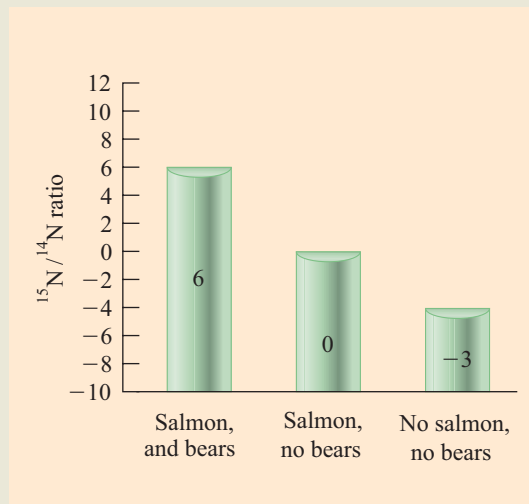
FIGURE 3.1 Nitrogen in trees near rivers with both salmon and bears have a significantly higher ^{15}\text{N}/^{14}\text{N} ratio in their foliage than do trees with salmon and no bears, or those without either salmon or bears. These findings suggest an important role for both fish and bears in distributing marine-derived nitrogen in riparian forests.
