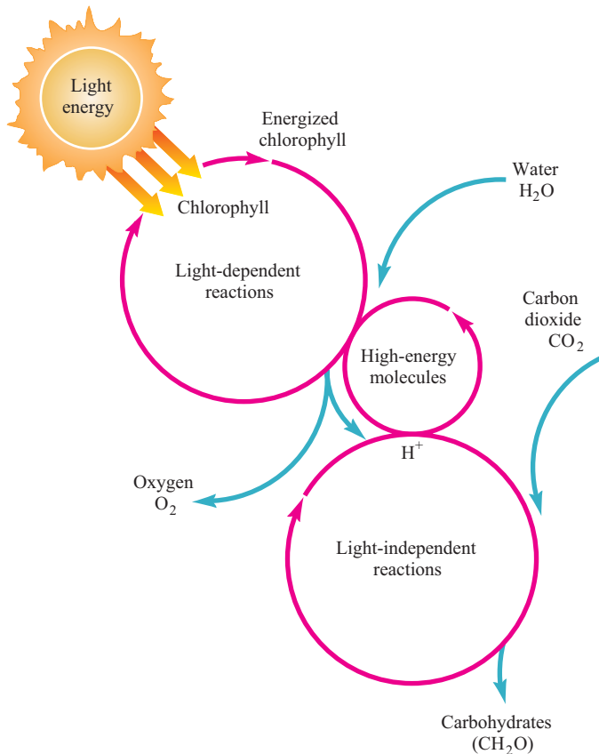
FIGURE 3.11 Photosynthesis involves a series of reactions in which chlorophyll captures light energy and forms high-energy molecules, ATP and NADPH. Light-independent reactions then use energy from ATP and NADPH to fix carbon (from air) in organic molecules.
