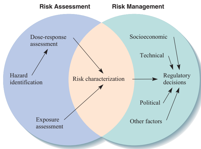
FIGURE 8.19 Risk assessment organizes and analyzes data to determine relative risk. Risk management sets priorities and evaluates relevant factors to make regulatory decisions.
