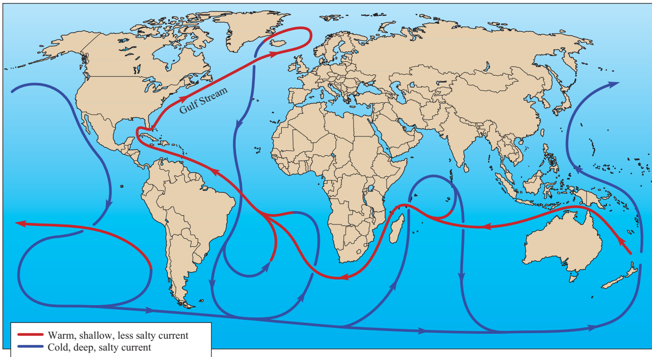
FIGURE 17.4 Ocean currents act as a global conveyor system, redistributing warm and cold water around the globe. These currents moderate our climate. For example, the Gulf Stream keeps northern Europe much warmer than northern Canada.
