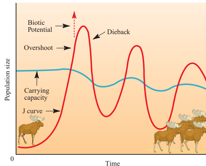
FIGURE 6.5 J curve, or exponential growth curve, with overshoot of carrying capacity. Exponential growth in an unrestrained population ( left side of curve ) leads to a population crash and oscillations below former levels. After the overshoot, carrying capacity may be reduced because of damage to the resources of the habitat. Moose on Isle Royale in Lake Superior may be exhibiting this growth pattern in response to their changing environment.
