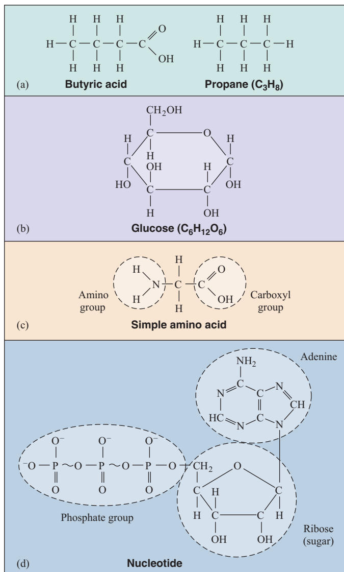
FIGURE 3.5 The four major groups of organic molecules are based on repeating subunits of these carbon-based structures. Basic structures are shown for (a) butyric acid (a building block of lipids) and a hydrocarbon, (b) a simple carbohydrate, (c) a protein, and (d) a nucleic acid.
