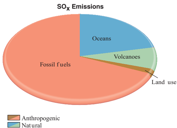
FIGURE 16.6 Sulfur fluxes into the atmosphere.
