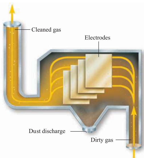
FIGURE 16.29 An electrostatic precipitator traps particulate material on electrically charged plates as effluent makes its way to the smokestack.
