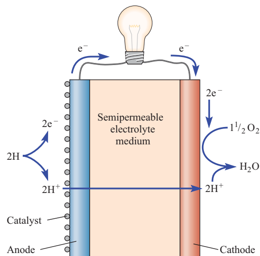
FIGURE 20.15 Fuel cell operation. Electrons are removed from hydrogen atoms at the anode to produce hydrogen ions (protons) that migrate through a semipermeable electrolyte medium to the cathode, where they reunite with electrons from an external circuit and oxygen atoms to make water. Electrons flowing through the circuit connecting the electrodes create useful electrical current.
