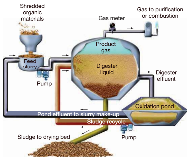
FIGURE 20.20 Continuous unit for converting organic material to methane by anaerobic fermentation. One kilogram of dry organic matter will produce 1–1.5 m 3 of methane, or 2,500–3,600 million calories per metric ton.
