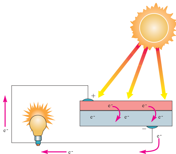
FIGURE 20.12 The operation of a photovoltaic cell. Boron impurities incorporated into the upper silicon crystal layers cause electrons ( e^- ) to be released when solar radiation hits the cell. The released electrons move into the lower layer of the cell, thus creating a shortage of electrons, or a positive charge, in the upper layer and an oversupply of electrons, or negative charge, in the lower layer. The difference in charge creates an electric current in a wire connecting the two layers.
