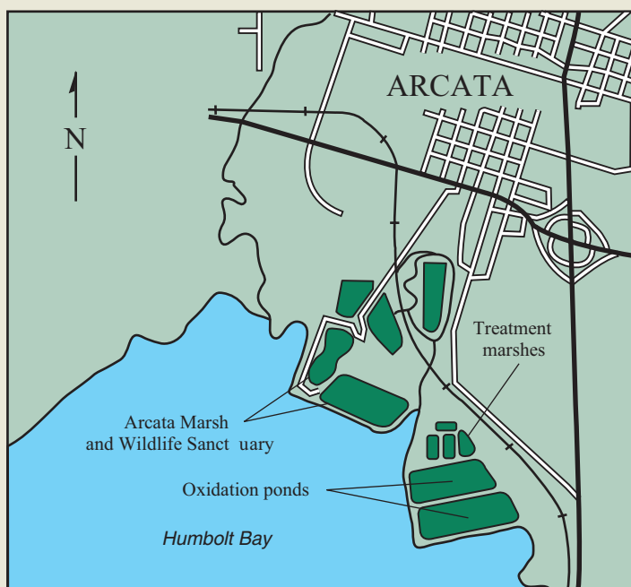
FIGURE 18.1 Arcata's constructed wetlands remove pathogens, pollutants, and nutrients from municipal wastewater using native biological communities and ecological processes in a setting that also serves as a wildlife sanctuary and tourist attraction.
