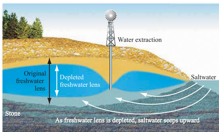
FIGURE 17.18 Saltwater intrusion into a coastal aquifer as the result of groundwater depletion. Many coastal regions of the United States are losing freshwater sources due to saltwater intrusion.
