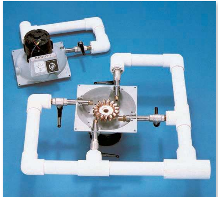
FIGURE 20.26 Solar collectors capture power only when the sun shines, but hydropower is available 24 hours a day. Small turbines such as this one can generate enough power for a single-family house with only 15 m (50 ft) of head and 200 l (50 g) per minute flow. The turbine can have up to four nozzles to handle greater water flow and generate more power.
