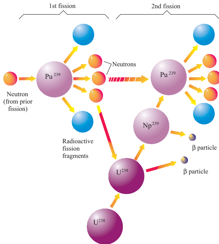
FIGURE 19.24 Reactions in a “breeder” fission process. Neutrons from a plutonium fission change U^{238} to U^{239} and then to Pu^{239} so that the reactor creates more fuel than it uses.
