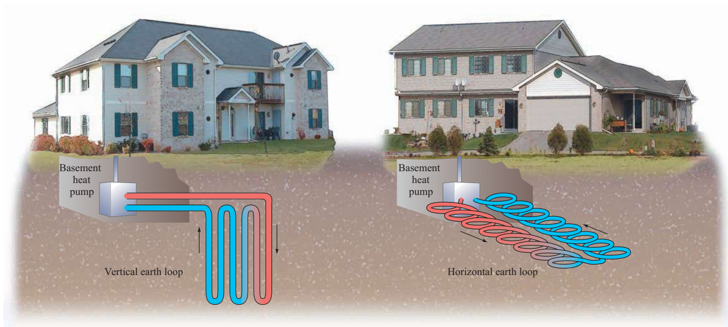
FIGURE 20.30 Geothermal energy can cut heating and cooling costs by half in many areas. In summer (shown here), warm water is pumped through buried tubing (earth loops) where it is cooled by constant underground temperatures. In winter, the system reverses and the relatively warm soil helps heat the house. Where space is limited ( left ), earth loops can be vertical. If more space is available ( right ) the tubing can be laid in shallow horizontal trenches. A heat exchanger concentrates heat, so water entering the house is far warmer than the ground temperature.
