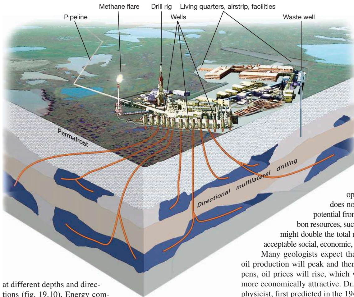
FIGURE 19.10 Horizontal, or directional drilling allows wells to extend up to 6 km horizontally from the well head. Up to 50 individual wells can be drilled from a single rig to reach isolated oil pockets.
