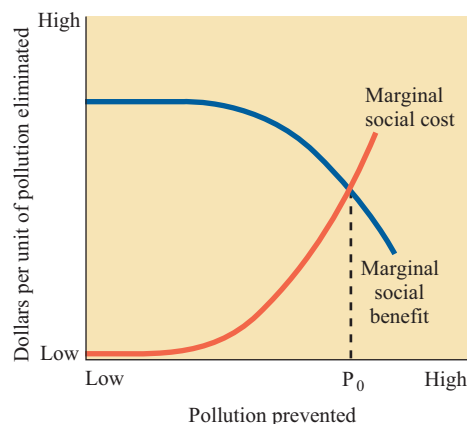
FIGURE 23.19 To achieve maximum economic efficiency, regulations should require pollution prevention up to the optimum point ( P_0 ) at which the costs of eliminating pollution just equal the social benefits of doing so.
