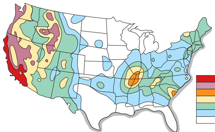
FIGURE 14.18 A seismic map of the lower 48 states shows the risk of earthquakes. Although the highest risk is along the Pacific coast and the Rocky Mountains, you may be surprised to see that an area along the Mississippi River around New Madrid, Missouri, also has a high potential for seismic activity.
