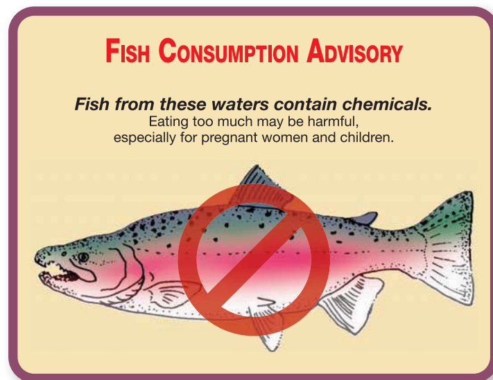
FIGURE 18.12 Mercury contamination is the second most common cause of impairment of U.S. rivers and lakes. Forty-five states have issued warnings about eating locally caught freshwater fish. Long-lived, top predators are especially likely to bioaccumulate toxic concentrations of mercury. The largest source of this highly dangerous toxin is coal-fired power plants.
