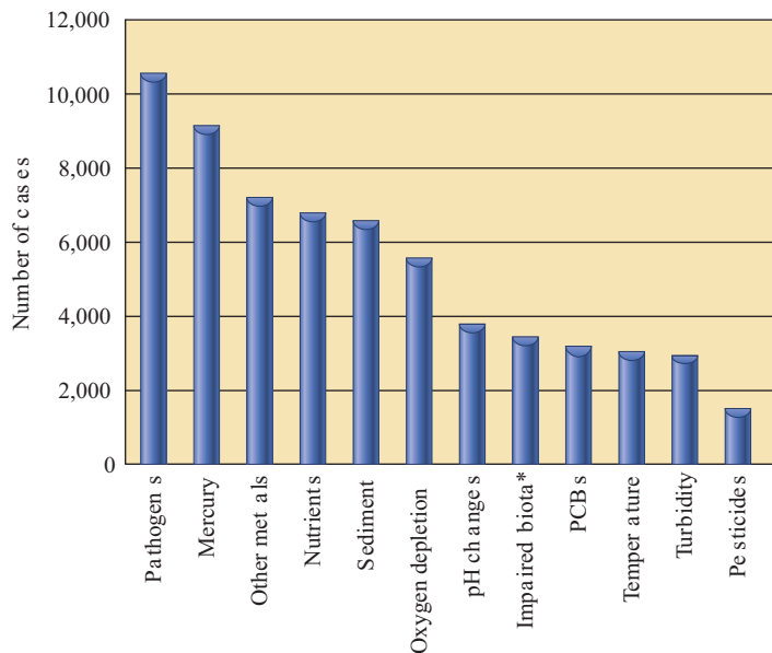
FIGURE 18.13 Twelve leading causes of surface-water impairment in the United States. *Undetermined causes.
