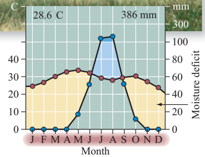
FIGURE 5.6 Tropical savannas and grasslands experience annual drought and rainy seasons and year-round warm temperatures. Thorny acacias and abundant grazers thrive in this savanna. Yellow areas show moisture deficit.
