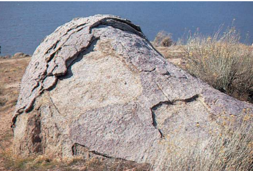
FIGURE 14.9 Weathering slowly reduces an igneous rock to loose sediment. Here, exposure to moisture expands minerals in the rock, and frost may also force the rock apart.
