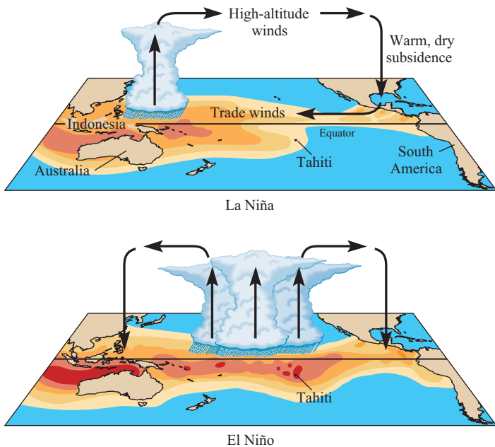
FIGURE 15.16 The El Niño/La Niña Southern Oscillation Cycle. During El Niño years, surface trade winds that normally push warm water westward toward Indonesia weaken and allow this pool of water to flow eastward, bringing storms to the Americas.
