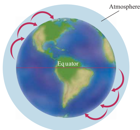
FIGURE 16.17 Air pollutants evaporate from warmer areas and then condense and precipitate in cooler regions. Eventually, this “grasshopper” redistribution leads to accumulation in the Arctic and Antarctic.
