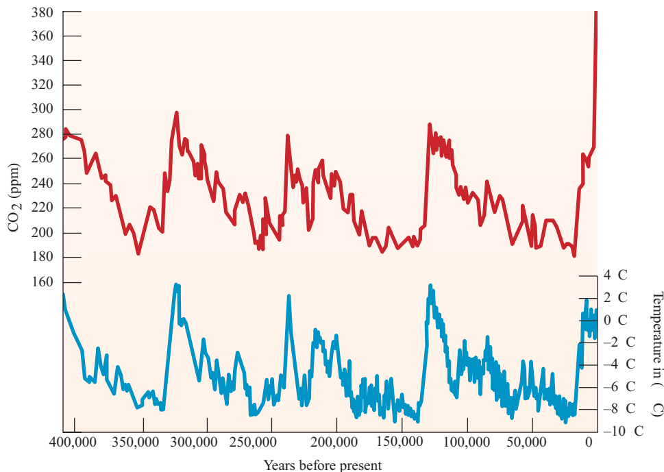
FIGURE 15.14 Atmospheric CO 2 concentrations and global mean temperatures estimated from the antarctic Vostok ice core. Note the relatively rapid changes and close correlation in both climate and atmospheric chemistry.
