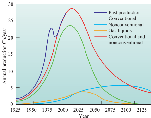
FIGURE 19.11 Worldwide production of crude oil with predicted Hubbert production. Gb = billion barrels.
