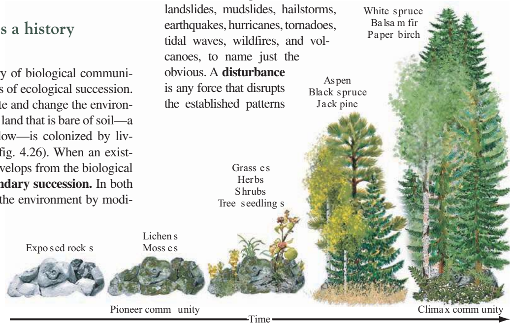
FIGURE 4.26 One example of primary succession, shown in five stages (left to right). Here, bare rocks are colonized by lichens and mosses, which trap moisture and build soil for grasses, shrubs, and eventually trees.
