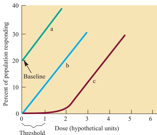
FIGURE 8.17 Three possible dose-response curves at low doses. (a) Some individuals respond, even at zero dose, indicating that some other factor must be involved. (b) Response is linear down to the lowest possible dose. (c) Threshold must be passed before any response is seen.
