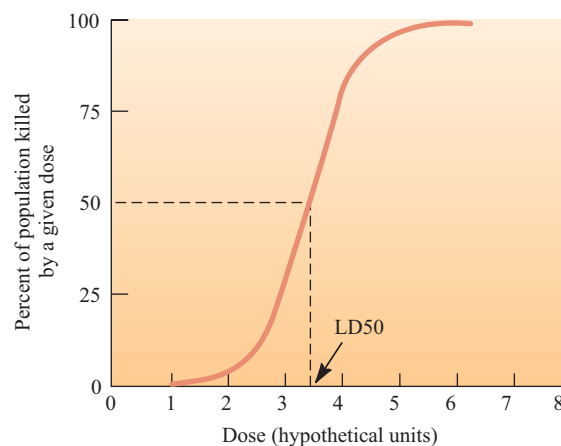
FIGURE 8.16 Cumulative population response to increasing doses of a toxin. The LD50 is the dose that is lethal to half the population.
