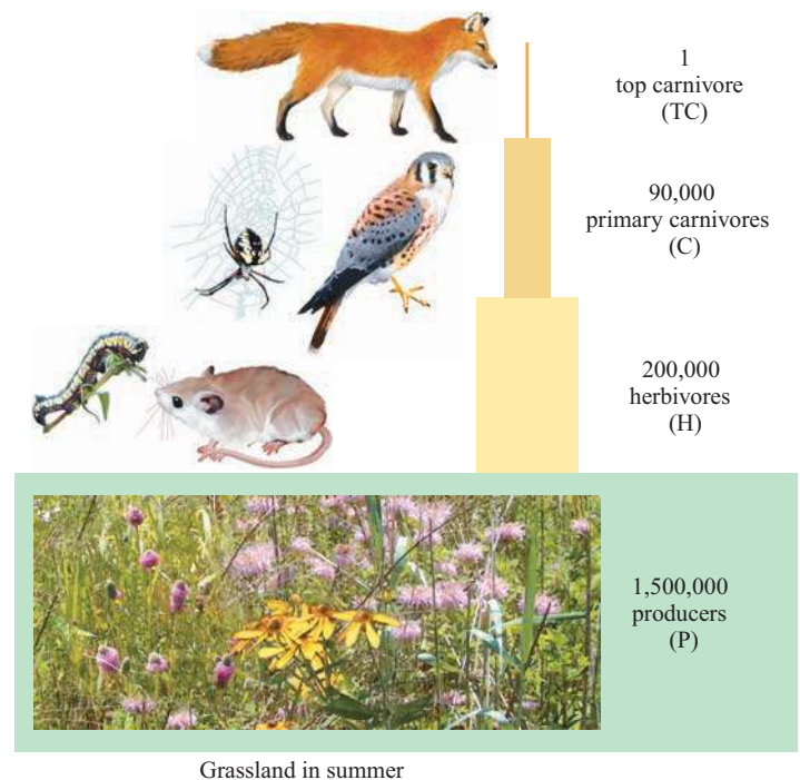
FIGURE 3.18 Usually, smaller organisms are eaten by larger organisms and it takes numerous small organisms to feed one large organism. The classic study represented in this pyramid shows numbers of individuals at each trophic level per 1,000 m 2 of grassland, and reads like this: to support one individual at the top carnivore level, there were 90,000 primary carnivores feeding upon 200,000 herbivores that in turn fed upon 1,500,000 producers.
