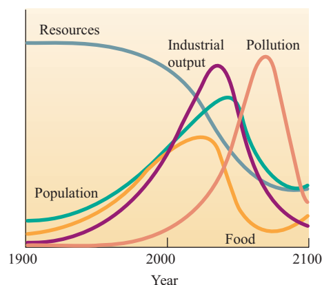
FIGURE 23.15 A run of one of the world models in Limits to Growth . This model assumes business-as-usual for as long as possible until Malthusian limits cause industrial society to crash. Notice that pollution continues to increase well after industrial output, food supplies, and population have all plummeted.
