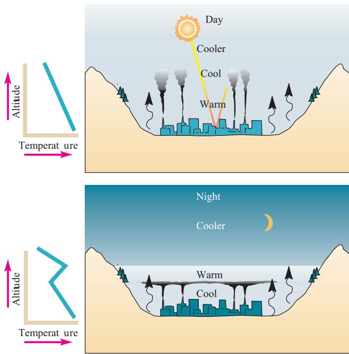
FIGURE 16.15 Atmospheric temperature inversions occur where ground level air cools more quickly than upper levels. This temperature differential prevents mixing and traps pollutants close to the ground.
