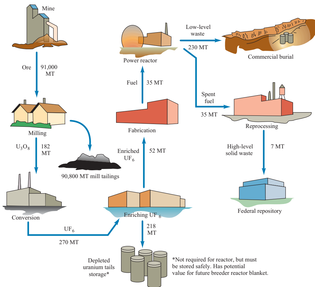
FIGURE 19.21 The nuclear fuel cycle. Quantities represent the average annual fuel requirements for a typical 1,000 MW light water reactor (MT = metric tons). About 35 MT or one-third of the reactor fuel is replaced every year. Reprocessing is not currently done in the United States.
