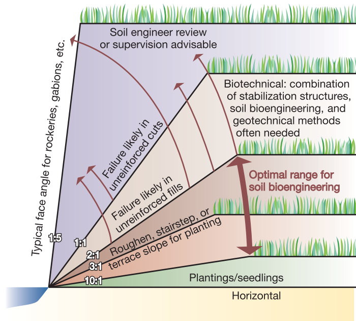
FIGURE 13.33 Steep streambanks need to be reinforced or recontoured to avoid erosion. Shallow slopes can be stabilized with vegetation or mulch. Steeper slopes need stabilization structures or reinforcement to hold the soil.
