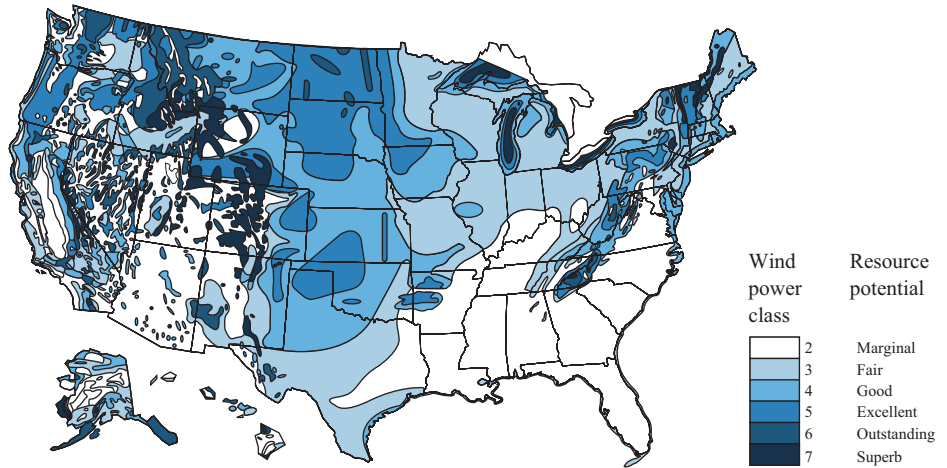
FIGURE 20.28 United States wind resource map. Mountain ranges and areas of the High Plains have the highest wind potential, but much of the country has a fair to good wind supply.
