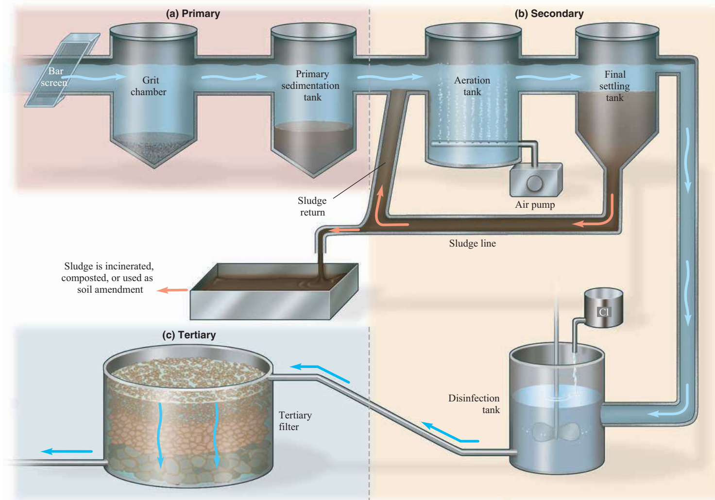
FIGURE 18.23 (a) Primary sewage treatment removes only solids and suspended sediment. (b) Secondary treatment, through aeration of activated sludge (or biosolids), followed by sludge removal and chlorination of effluent, kills pathogens and removes most organic material. (c) During tertiary treatment, passage through a trickling bed evaporator and/or a lagoon or marsh further removes inorganic nutrients, oxidizes any remaining organics, and reduces effluent volume.
