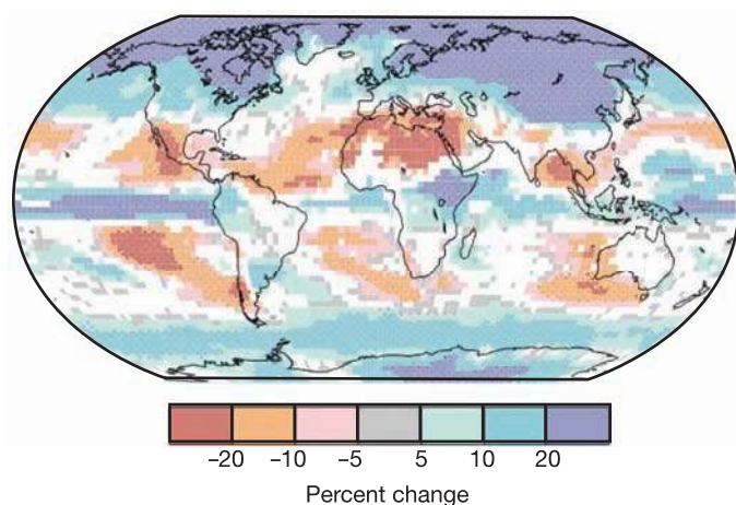
FIGURE 17.19 Relative changes in precipitation (in percentage) for the period 2090–2099 compared to 1980–1999, predicted by the Intergovernmental Panel on Climate Change. Source: IPCC, 2007.
