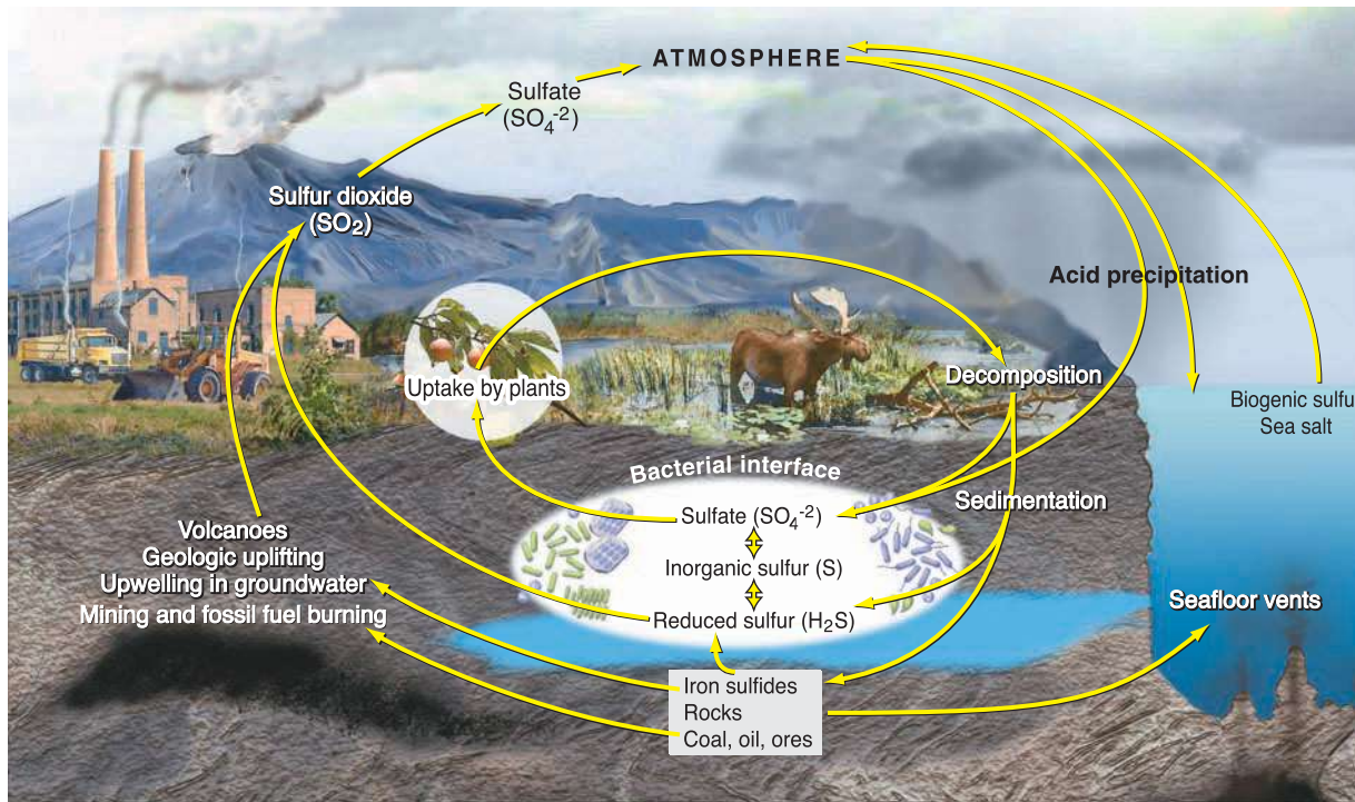
FIGURE 3.24 The sulfur cycle. Sulfur is present mainly in rocks, soil, and water. It cycles through ecosystems when it is taken in by organisms. Combustion of fossil fuels causes increased levels of atmospheric sulfur compounds, which create problems related to acid precipitation.
