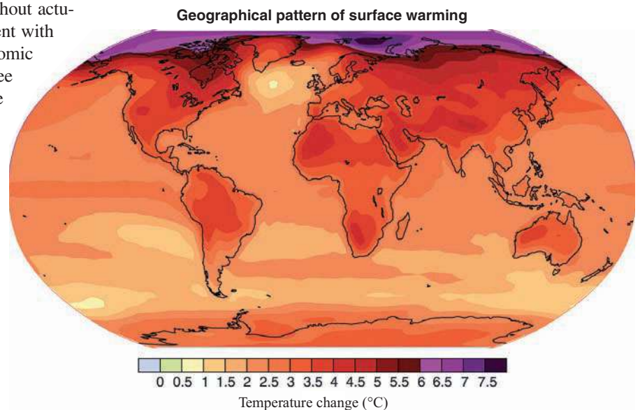
FIGURE 2.8 Numerical models, calculated from observed data, can project future scenarios. Here, temperature changes in 2090–2099 are modeled, relative to 1980–1999 temperatures.
