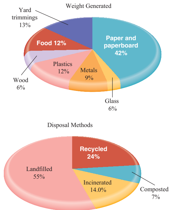
FIGURE 21.3 Composition of municipal solid waste in the United States by weight, before recycling, and disposal methods.
