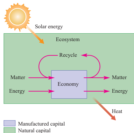
FIGURE 23.9 In natural resource economics, the economy is seen as an open subset of the ecosystem. Matter and energy are consumed in the form of raw resources and rejected as waste. Material is recycled by ecological processes, while heat is ejected back to space. Manufactured or “built” capital is regarded as scarce—and therefore valuable—while natural capital is regarded as plentiful and, therefore, cheap.
