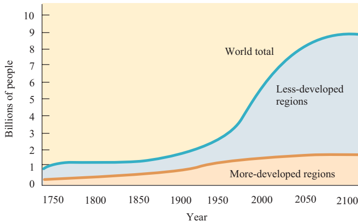
FIGURE 7.6 Estimated human population growth, 1750–2100, in less-developed and more-developed regions. Almost all growth projected for the twenty-first century is in the less-developed countries.
