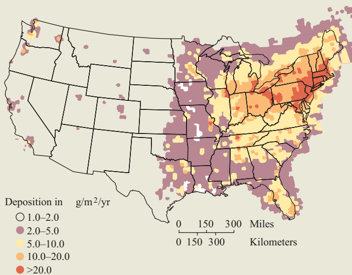
FIGURE 16.1 Atmospheric mercury deposition in the United States. Due to prevailing westerly winds, and high levels of industrialization, eastern states have high mercury deposition.
