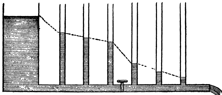
FIG. 53—PHYSICAL MODEL
