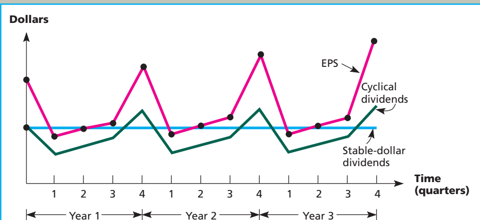
FIGURE 18.5 Alternative Dividend Policies for Big Department Stores, Inc.
