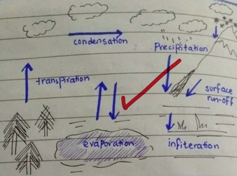
Fig 1 : Hydrological Cycle
